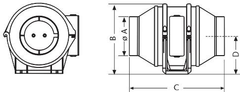
DUCT IN-LINE 150-200
