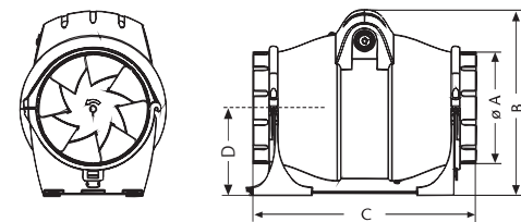
DUCT IN-LINE 150-200
